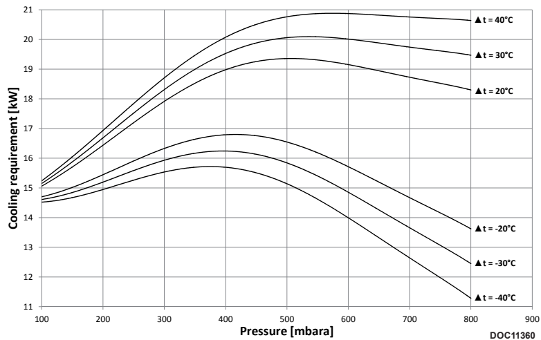
KL430 - 1750 rpm - Vacuum
