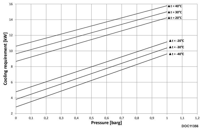
KL350 - 1750 rpm - Pressure
