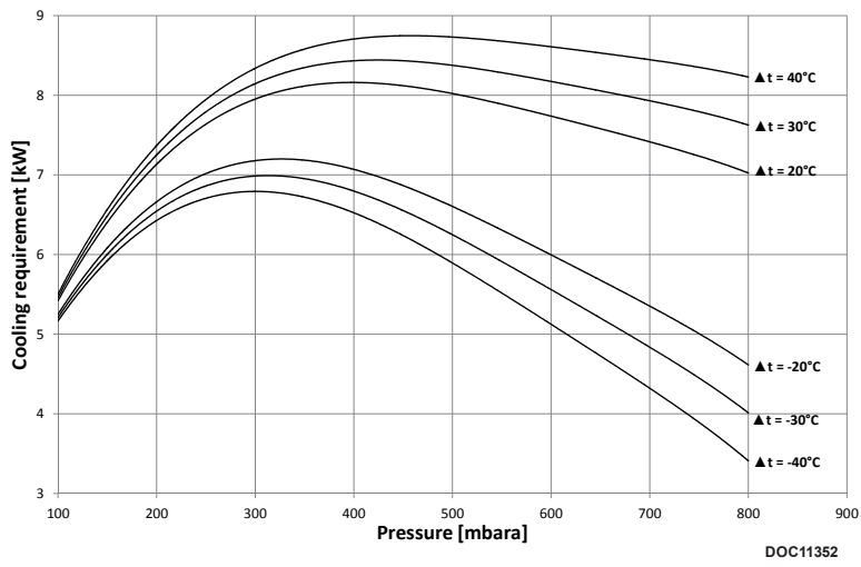
KL350 - 1450 rpm - Vacuum
